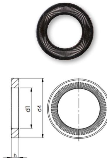
Backup Washer
